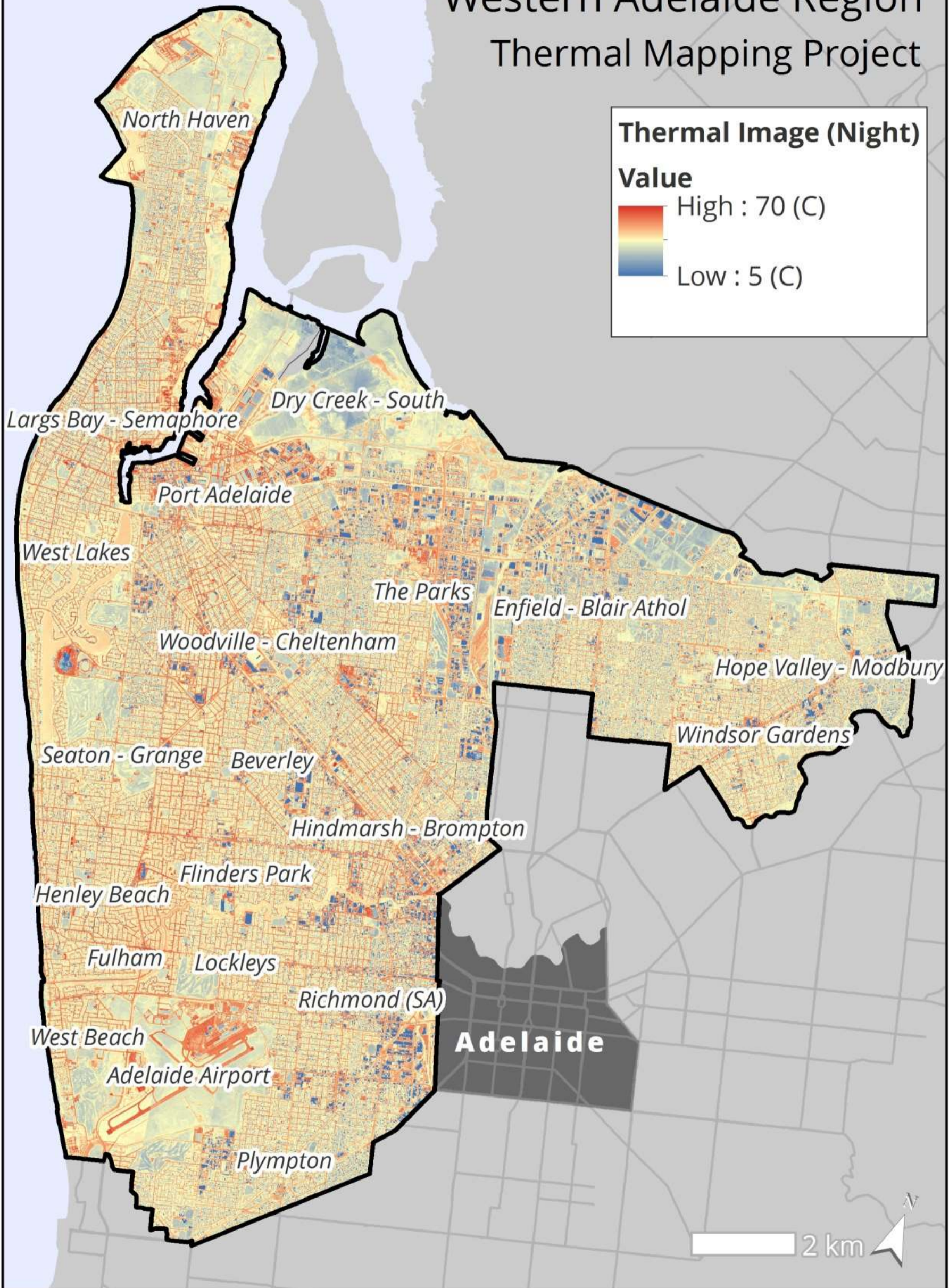
Figure 3. Night time thermal map showing the surface temperature for different features in the landscape at 2 m resolution for the Western Adelaide Region.
