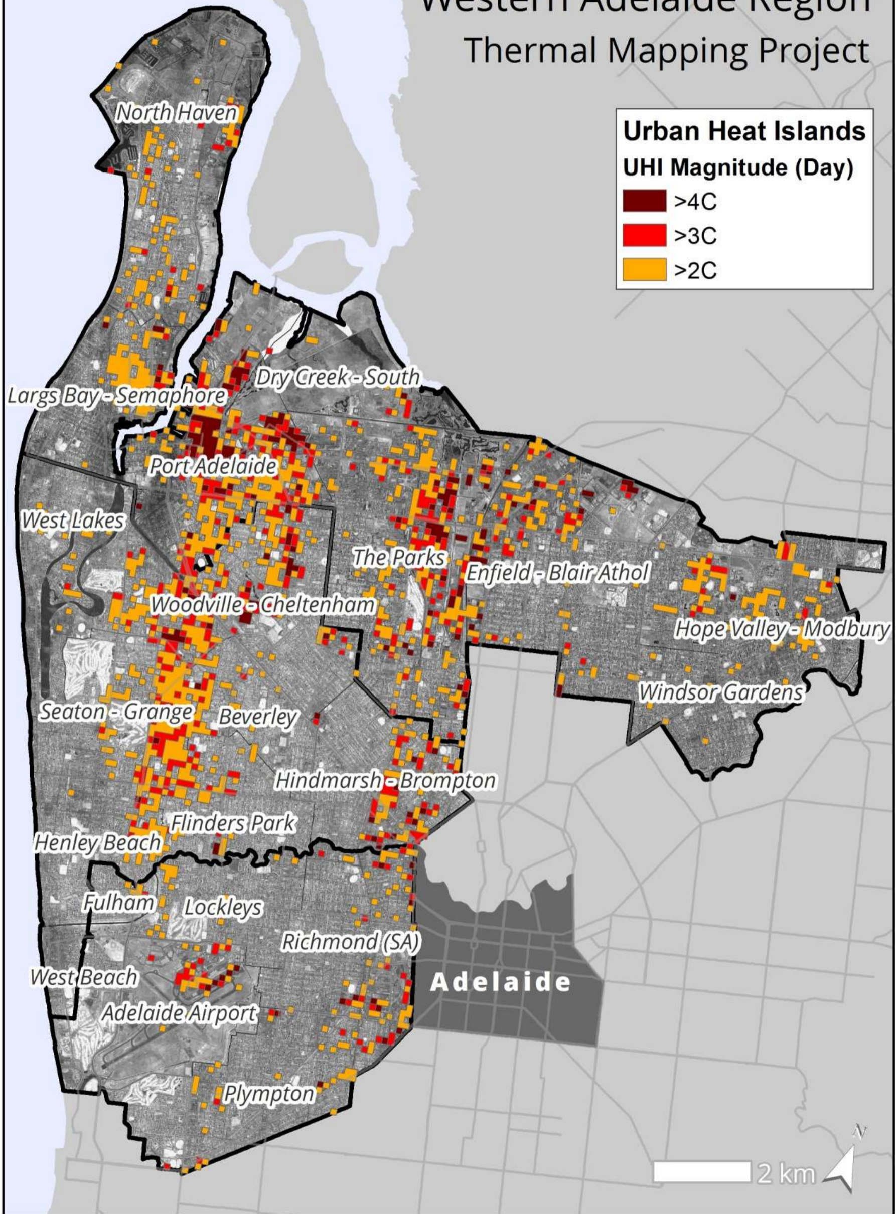
Figure 4. Daytime urban heat islands present in the Western Adelaide Region on 9 February 2017. Areas of built-up heat were identified as exhibiting a temperature greater than 2°C, 3°C or 4°C above the local mean temperature at the time of measurement.
