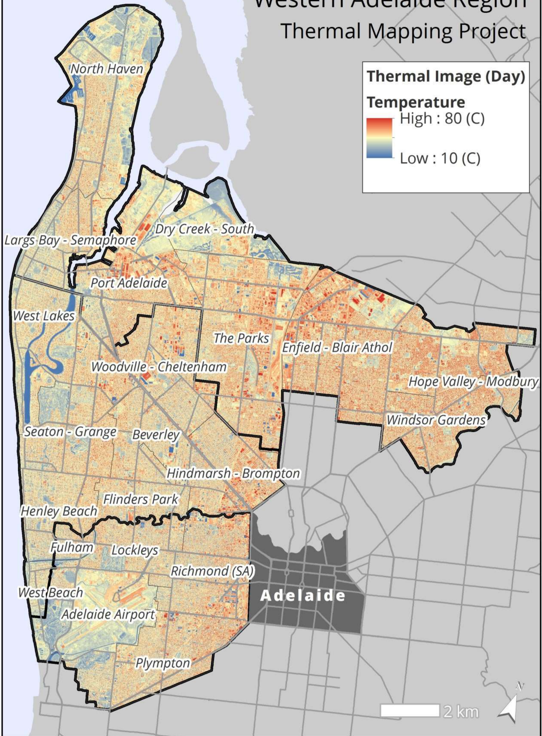
Figure 2. Day time thermal map showing the surface temperature for different features in the landscape at 2 m x 2 m resolution.
